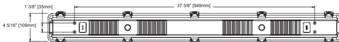
Top View
