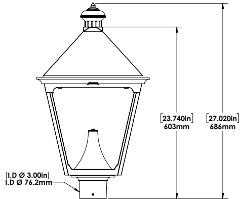
With Decorative Top (Standard)
