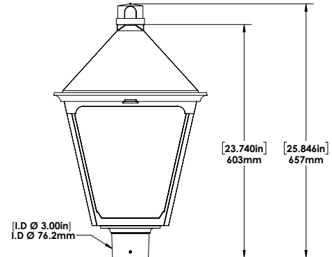
With Photocell (Option)
