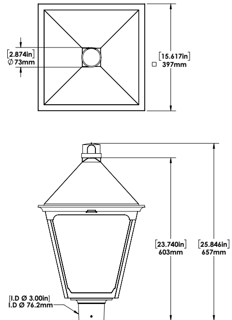
With Photocell (Option)
