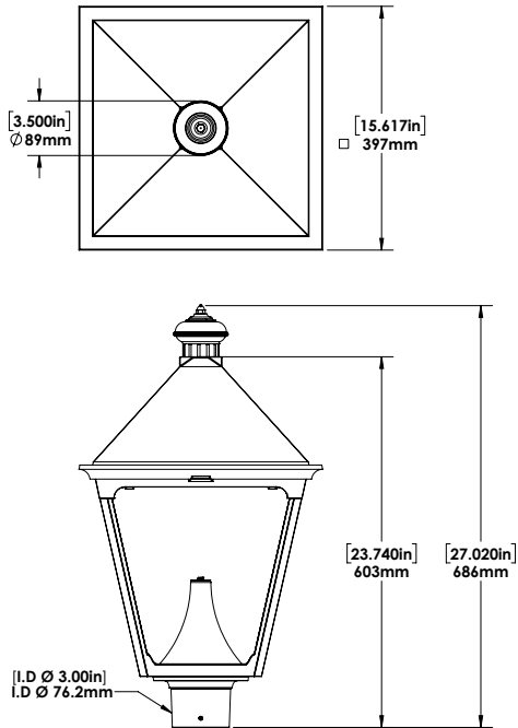
With Decorative Top (Standard)
