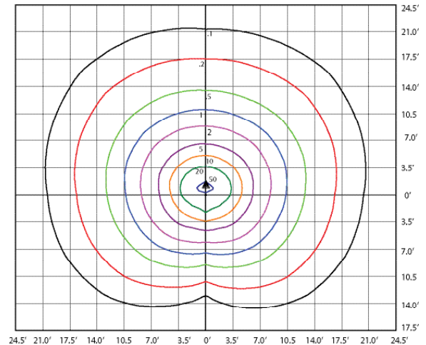
RAY8S-LED35-B-4K-270 DEGREE
