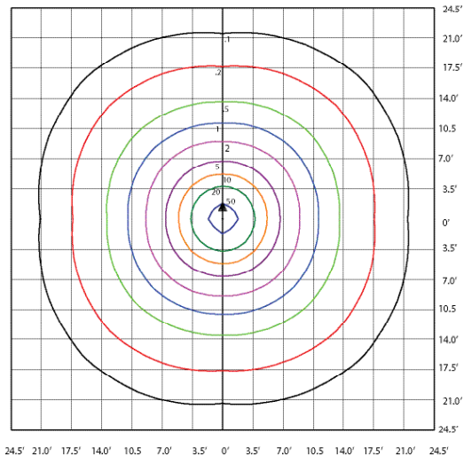
RAY8S-LED35-B-4K-360 DEGREE
