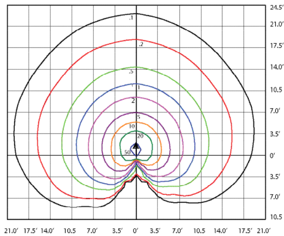
RAY8S-LED35-B-4K-180 DEGREE
