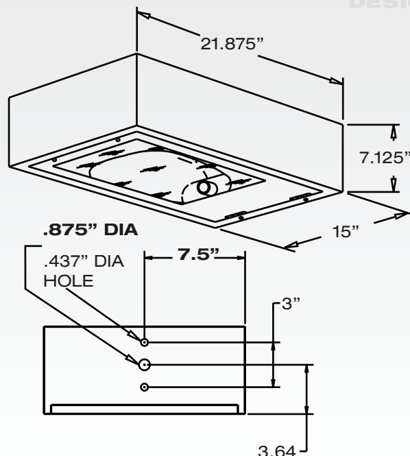
ARM DRILLING PATTERN
