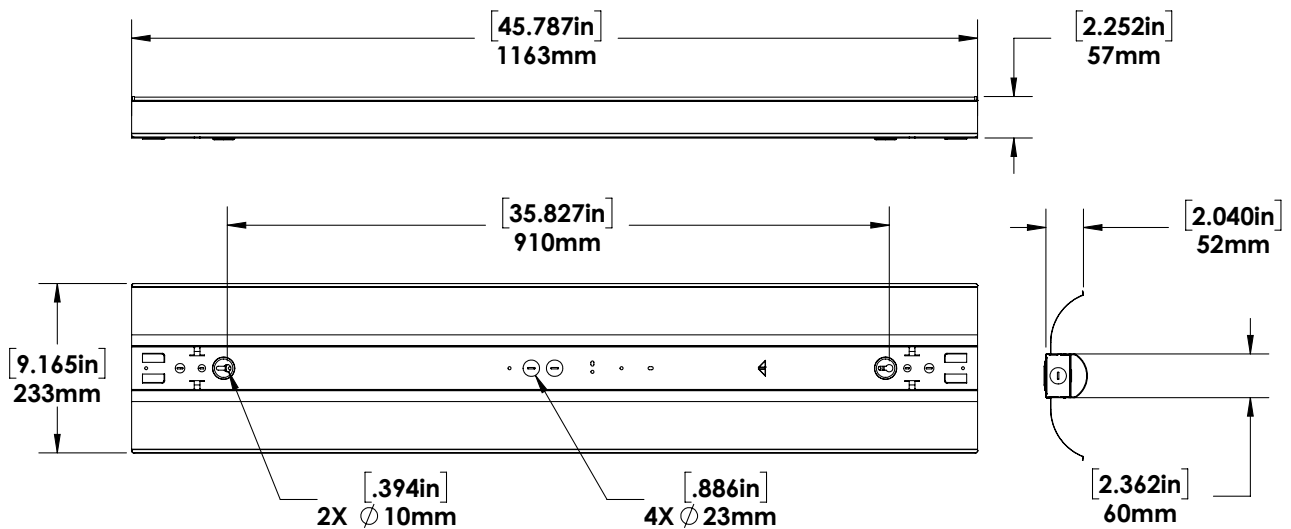
Wings on fixture dimensions
