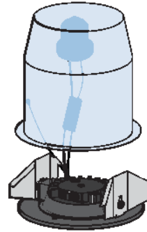
RECESSED HOUSING
