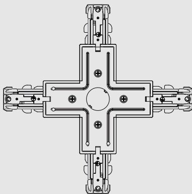
"X" Connector W 180 mm (7.09") x H 180 mm (7.09")
