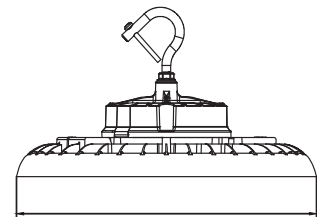
65-771R2: \varnothing 13.4" (340 \pm 5mm)
