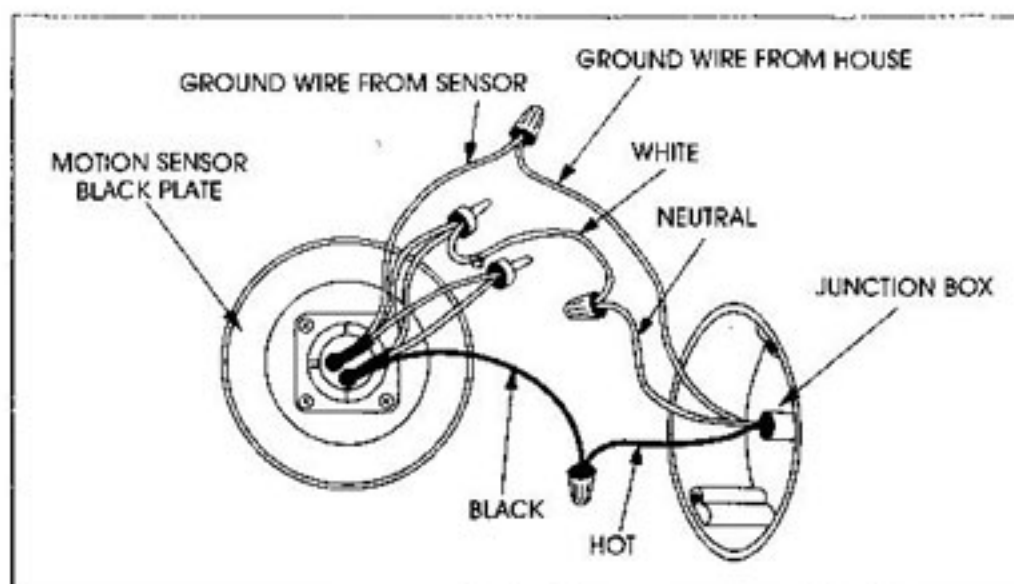
FIGURE 1: Installing the fixture
