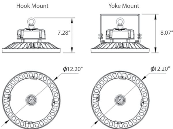
SSL-CHB/150M
